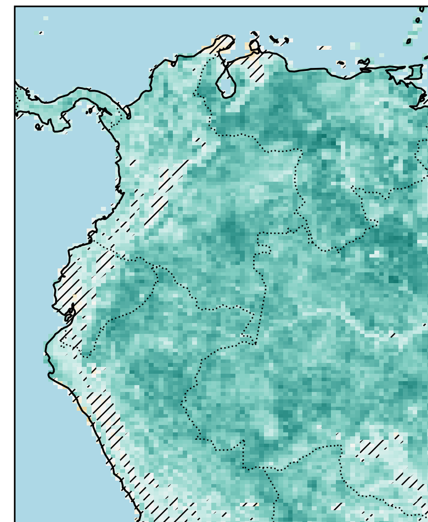
Average ( p = 8.37\text{e-}01 )
