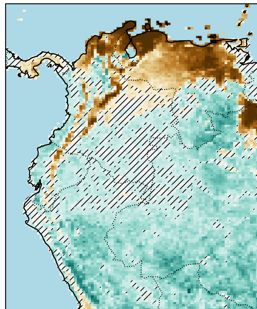
CCA ( p = 5.65\text{e-}03 )
